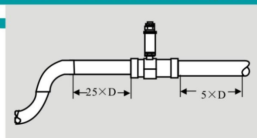
Two 90° elbows for one plane
