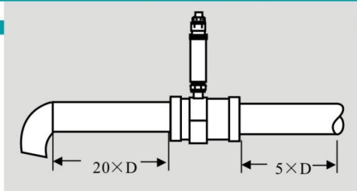
One 90° elbow
