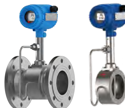
VFM60MV Multi-variable Vortex Meter standard type support up to 150 °C
